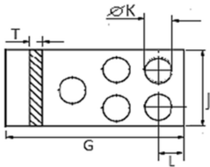
Top Busbar
