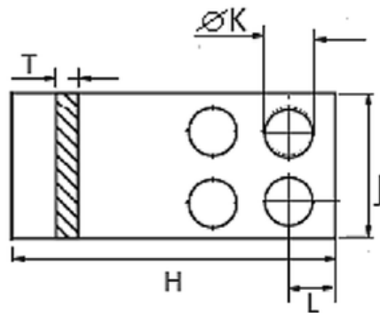
Bottom Busbar
