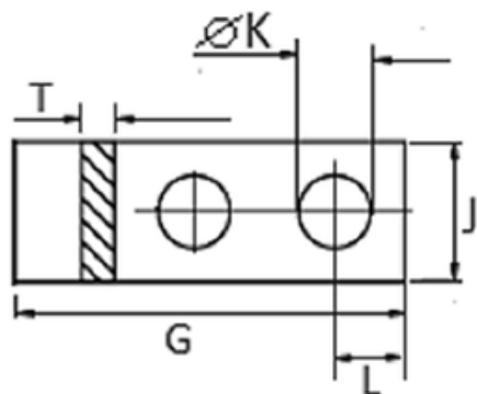
Top Busbar
