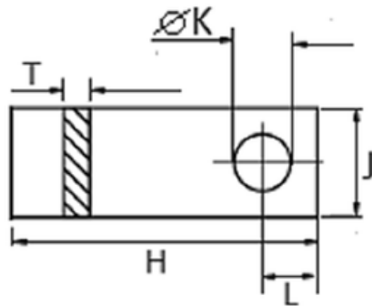
Bottom Busbar
