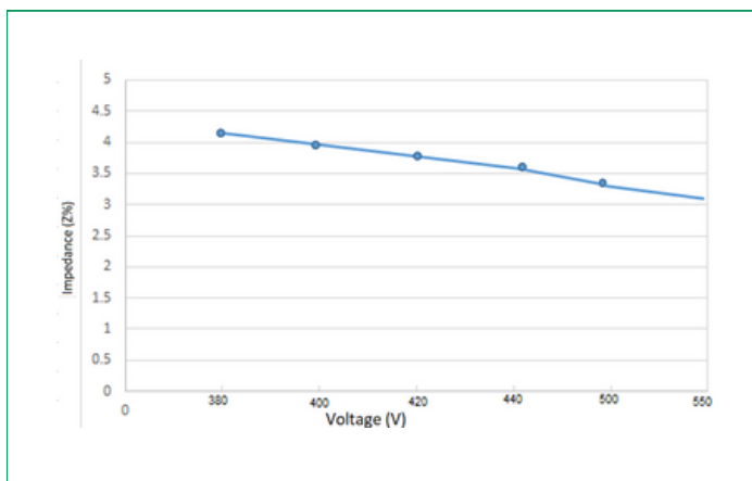
Impedance versus Voltage Plot
