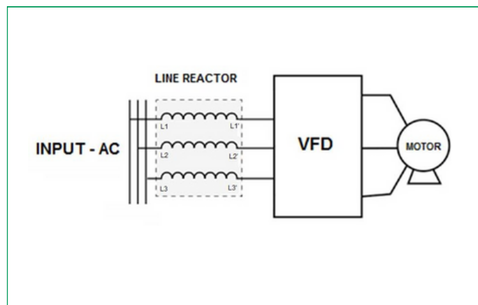
Connection Diagram
