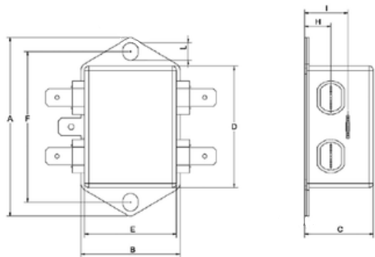
Connection Style - 04, 1A Type
