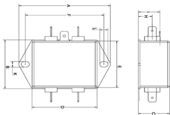
Connection Style - 04, 3A to 6A Type
