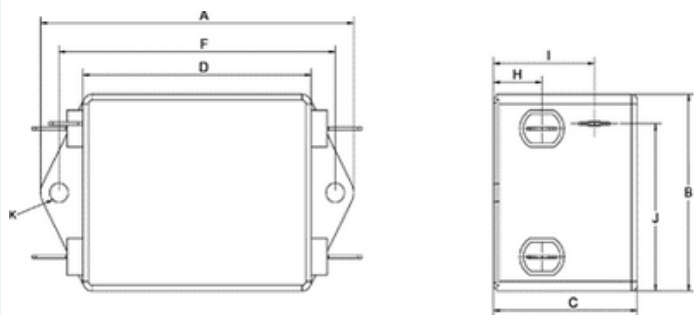
Connection Style - 04, 16A to 20A Type
