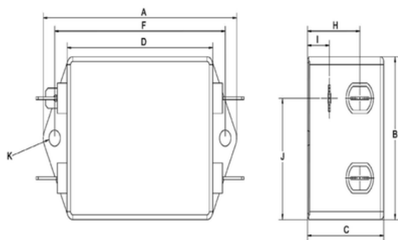
Connection Style - 04, 8A to 12A Type
